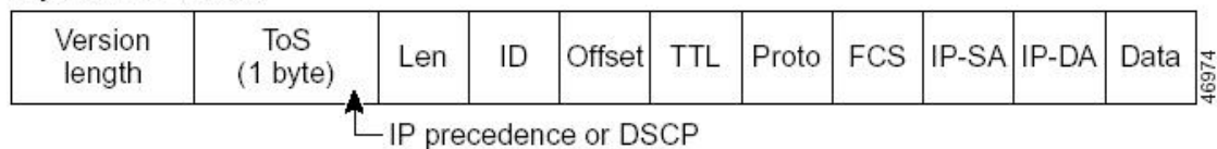
Diagram 10-2 ToS Priority
